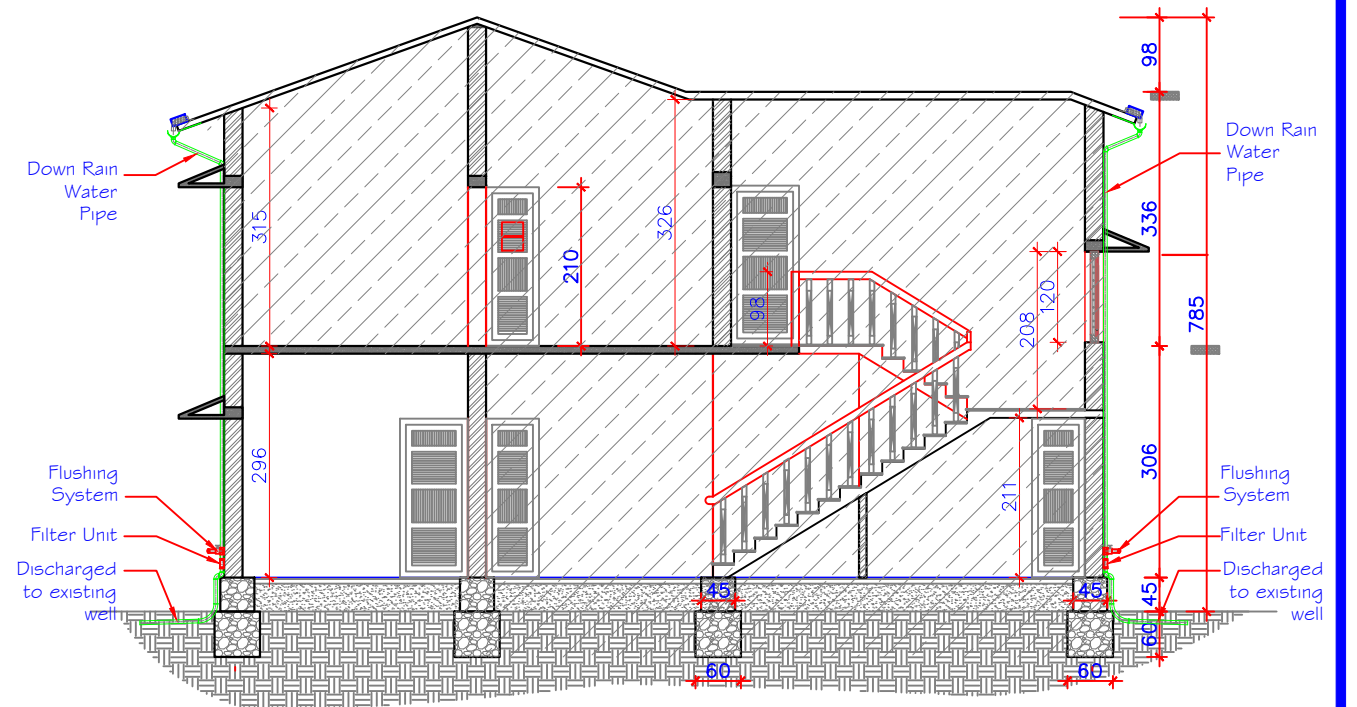
3 DETAILS FOR RAIN WATER DISCHARGING SYSTEM
