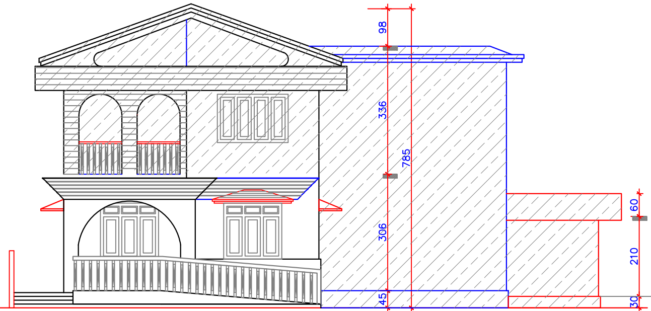
1 FRONT ELEVATION SCALE : 1:100
