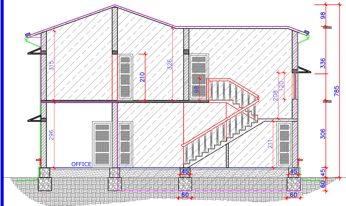
2 SECTION @ A SCALE : 1:100
